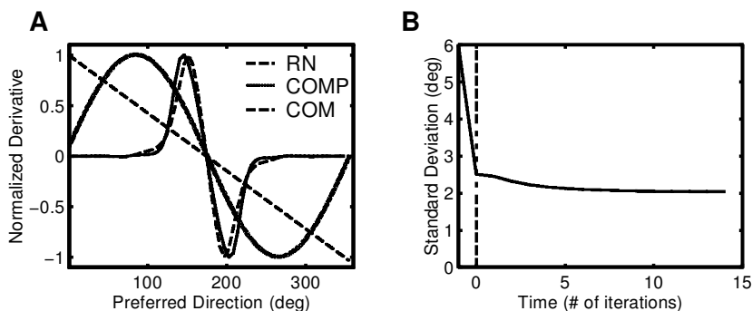
Figure 6: (A) Comparison of f'(\theta) (solid line) and -\partial\hat{\theta}/\partial a_i|_{\theta=170^\circ} for RN, COMP, and COM. All functions have been normalized to one. (B) Standard deviation as a function of time, or number of iterations of the recurrent network. The point at t = -1 is the COMP estimator applied to the input activity, A , whereas the point at t = 0 corresponds to COMP applied to WA .
