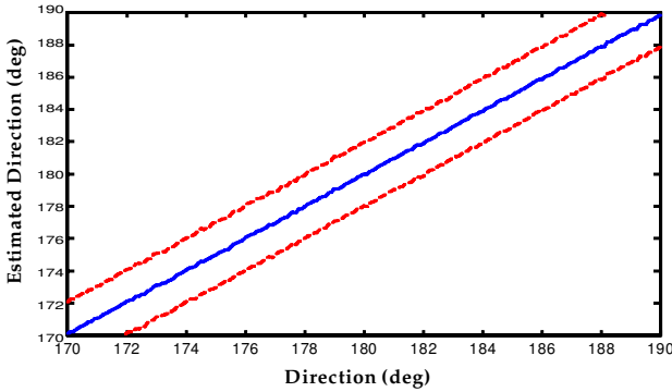
Figure 4: The solid line shows the mean estimated direction as a function of the true direction for normally distributed noise of fixed variance. The estimator is unbiased, that is, the mean estimate is equal to the true direction. The upper and lower dotted lines are one standard deviation away from the mean.
