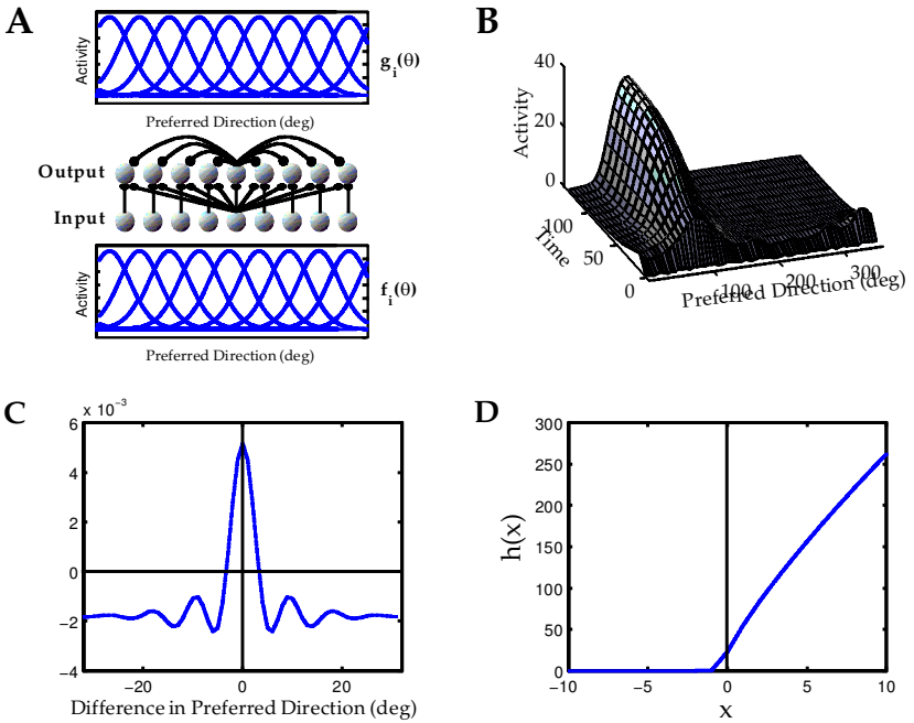
Figure 3: (A) Two-layer network for estimation using coarse code. The first layer generates the noisy activity pattern \{a_i\} according to the tuning function \{f_i(\theta)\} . The output layer is a recurrent network that generates a hill of activity corresponding to the tuning function \{g_i(\theta)\} . (B) Activity over time in the output layer with a nonlinear activation function in response to an initial small, random pattern of activity. The activity of the units is plotted as a function of their preferred direction of motion. (C) Pattern of weights in the nonlinear recurrent network as a function of the difference in preferred direction between units. (D) Activation function, h(x) , of the nonlinear recurrent network.
