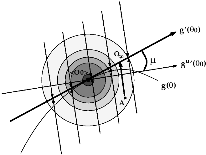
Figure 9: During relaxation, the initial activity A = O_0 is projected onto the tangent, \mathbf{g}'(\theta_0) , of the stable manifold defined by the function \mathbf{g}(\theta) , along directions orthogonal to \mathbf{g}''(\theta_0) . As a result, the initial distribution of activity (shown as a density plot indicated by the gray circles) is collapsed onto the axis defined by \mathbf{g}'(\theta_0) .
