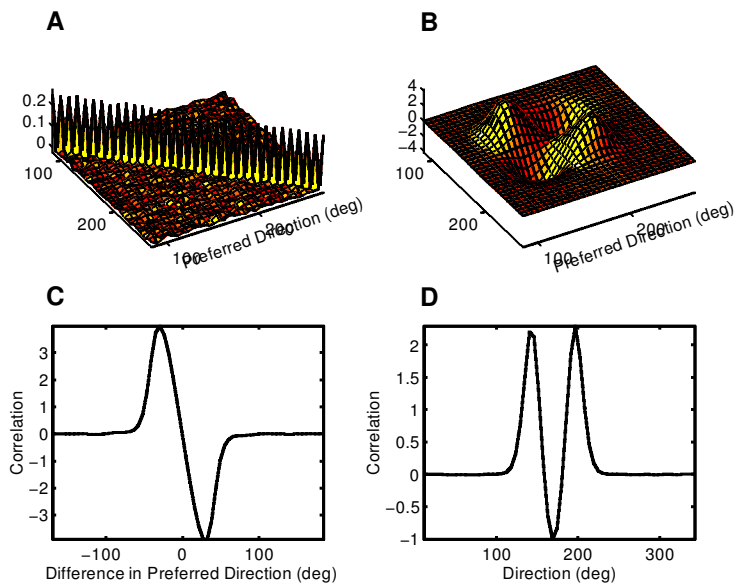
Figure 8: Covariance matrices of the input units (A) and network units (B) for repetitive presentations of a direction of 170 degrees. Only the central part of the covariance matrix is shown (units with preferred directions between 84 and 270 degrees). Whereas the input units are independent, the output units are correlated due to the lateral connections. (C) Correlation of unit with preferred direction 135 degrees with all the other units as a function of the difference in preferred direction. The curve has the same profile as the derivative of the tuning curve. (D) Correlation between two units (preferred directions 158 and 182 degrees) as a function of stimulus direction.
