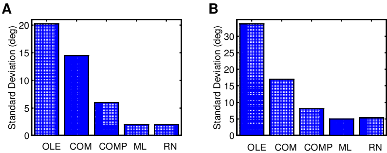
Figure 5: Histogram of the standard deviations of the estimate for all five methods (OLE, optimal linear estimator; COM, center of mass; COMP, complex estimator; ML, maximum likelihood; RN, recurrent network). (A) Noise with normal distribution. (B) Noise with Poisson distribution. In both cases, the value for ML is the Cramér-Rao bound. The RN method reaches this bound for gaussian noise and performs slightly worse for Poisson noise.
