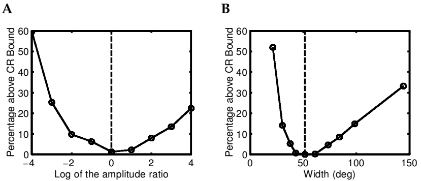
Figure 7: Standard deviation of the RN estimator in terms of percentage above the Cramér-Rao bound, as a function of the amplitude (A) and width (B) of the input bump. (A) The data are plotted as a function of the logarithm in base 2 of the ratio of input-output amplitudes. Changing the gain of the input by a factor of 2 or less affects the performance of the network only moderately. (B) The width of the tuning curve is computed at half the peak value. The network sharpens the input tuning curves for width values above 50 degrees and widens for smaller values. The Cramér-Rao bound is reached only when the widths of the input and output tuning curves differ by less than 10 degrees.
