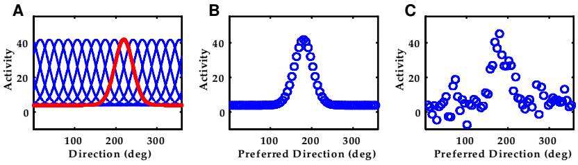
Figure 1: (A) Idealized tuning curves for 16 direction-tuned neurons. (B) Noiseless pattern of activity (o) from 64 simulated neurons with tuning curves like the ones shown in A, when presented with a direction of 180^\circ . (C) Same as in B but in the presence of gaussian noise.
