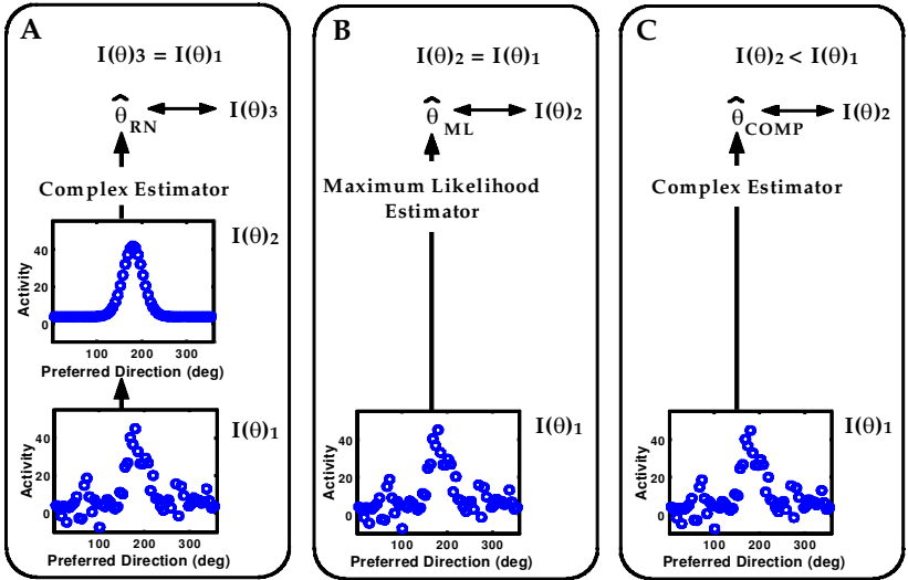
Figure 10: The COMP estimate preserves Fisher information, I(\theta)_1 , when applied to the stable hill of the recurrent network (A)—as ML does (B)—but not when applied to the initial input (C). Therefore, the network dynamics changes the format of information such that a simple estimator can read out the activity optimally. I(\theta)_1 , I(\theta)_2 , and I(\theta)_3 refer to the Fisher information about direction at various stages in the estimation process.
