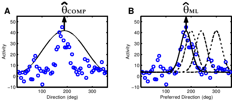
Figure 2: (A) The complex estimator uses the phase of the first Fourier component of the input pattern (solid line) as an estimate of direction. It is equivalent to fitting a cosine function to the input. (B) The ML estimate is found by moving an “expected” hill of activity (dotted line) until the squared distance with the data is minimized (solid line).
